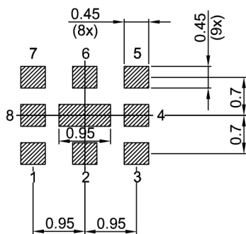
Figure 2: Drawing of package with package height A = 0.53 mm (max.). See Sec. Package information (p. 15).
